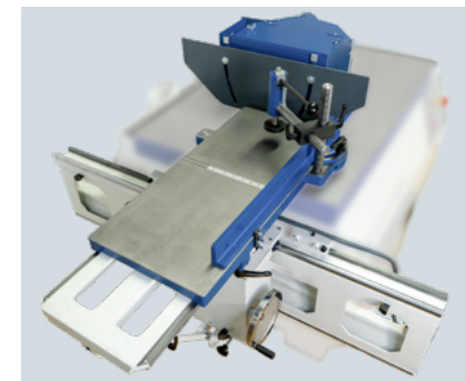
Sliding table with protective hood
