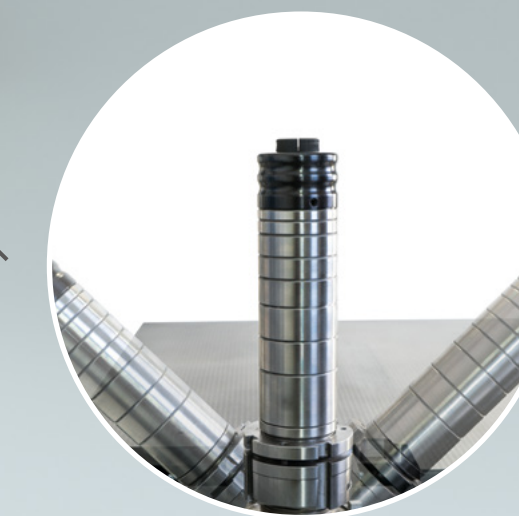
Rigid or swiveling spindle ( 45,5^\circ on both sides)
