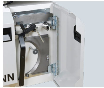
Tool deposit
