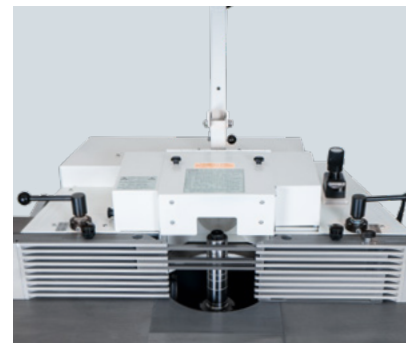
Fence type 2620 with integral fence jaws
