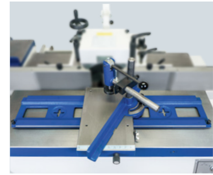
Sliding carriage
