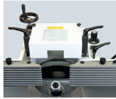
Fence type 2601 with integral fence jaws
