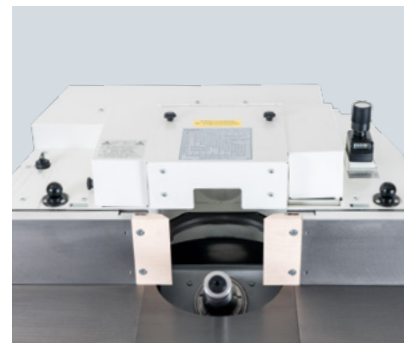
Fence type 2620 with air-lock and cast iron jaws
