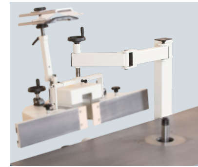
Swivel unit for fence
