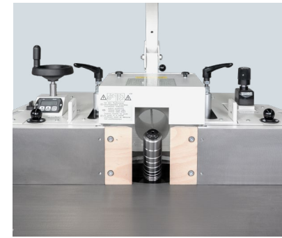
Fence type 2620 with cast fence jaws, AIR-LOCK
