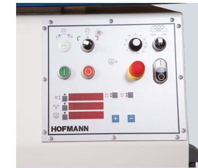
Control panel with variable spindle speed – with option of gradual feed speed
