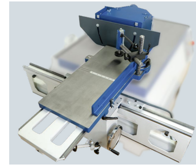
Rolling table with protective hood
