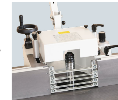
Fence type 2601 efficient with cast bolsters, safety rulers
